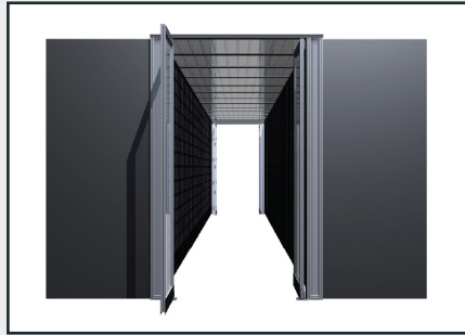
Cold aisle With Shrink-Away Ceiling and Pivot Doors
