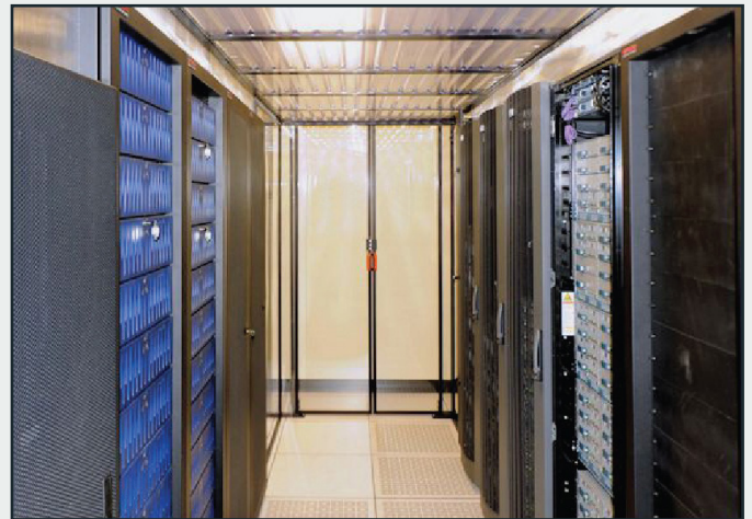
Shrink-Away Ceiling Variable Cabinet Height
